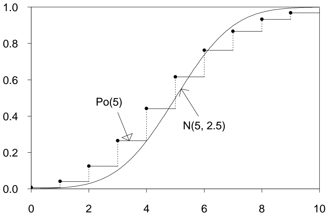
Cumulative Distributions: Normal and Poisson
