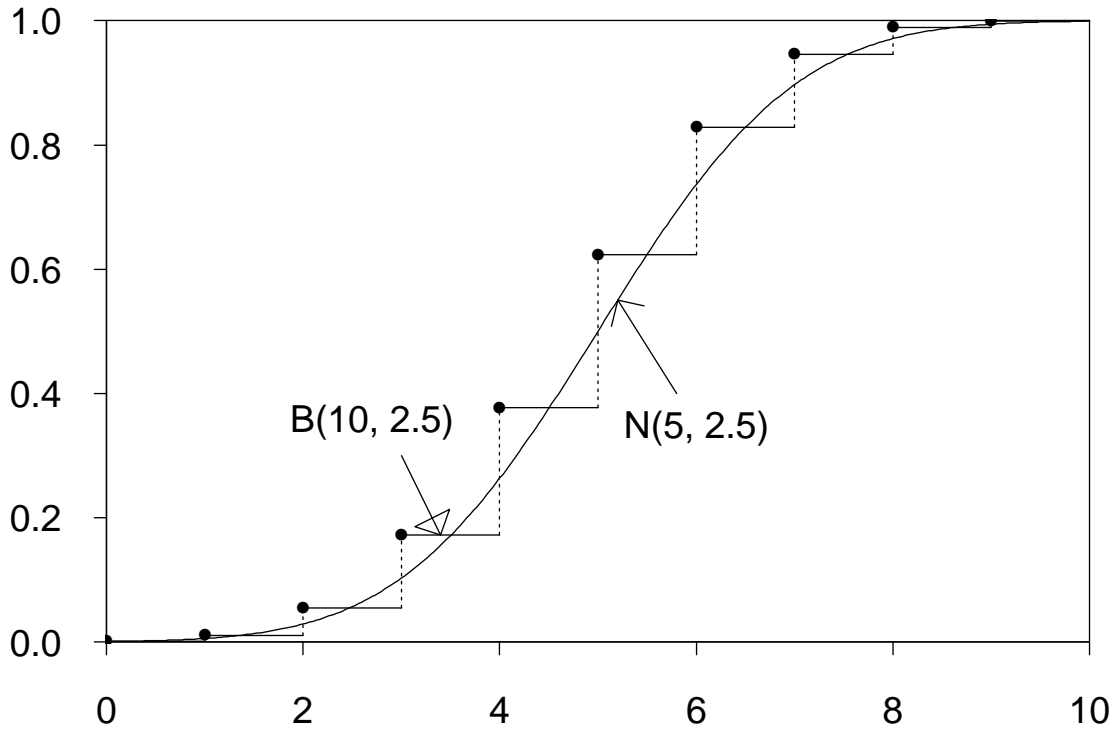
Cumulative Distributions: Normal and Binomial
