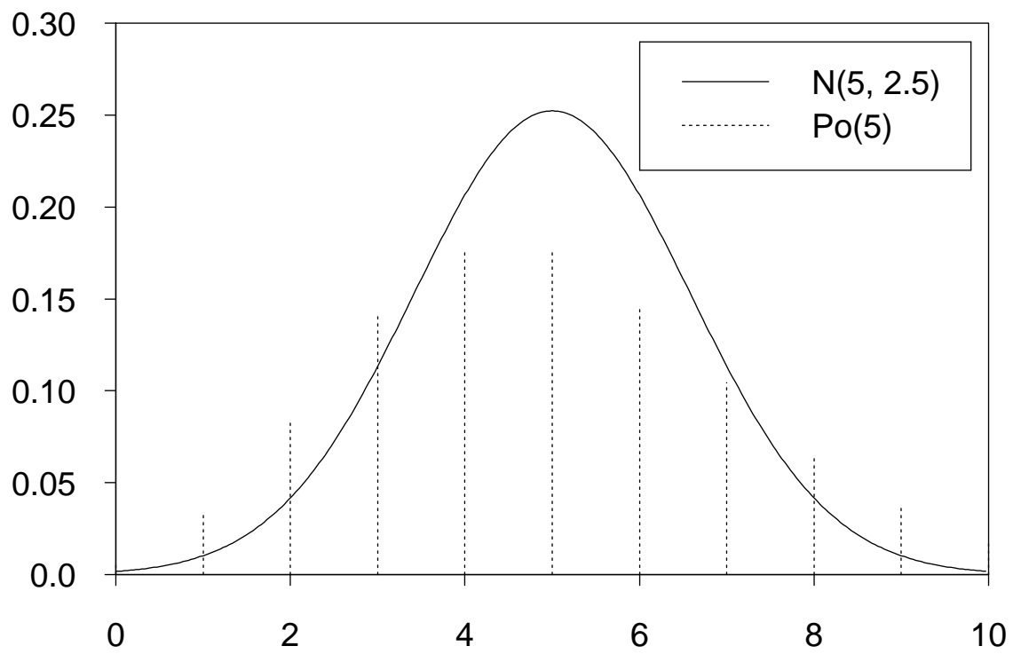
Probability Densities: Normal and Poisson
