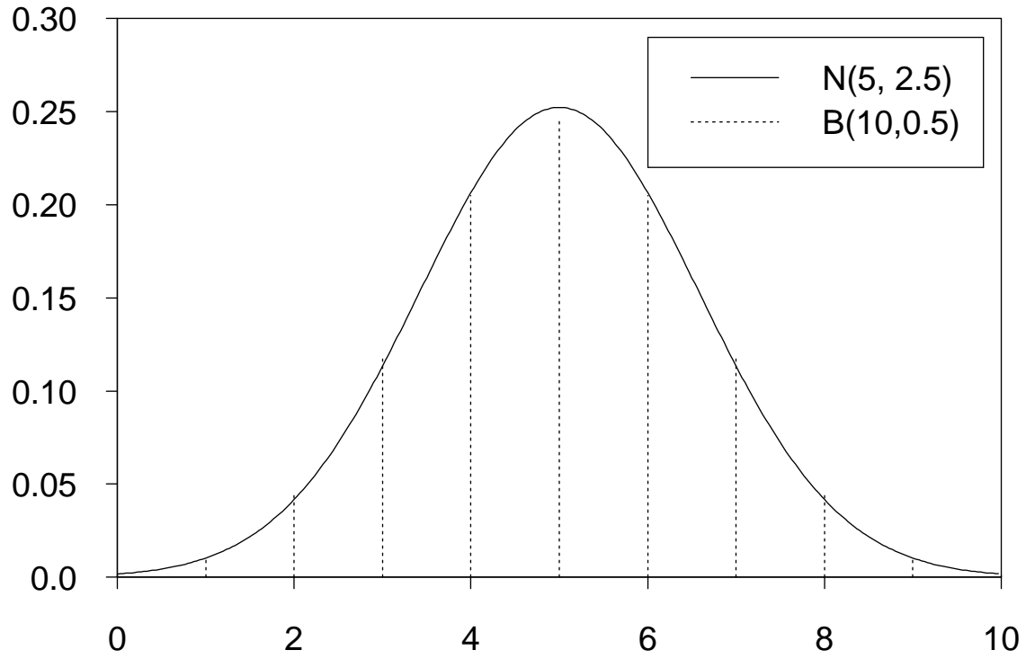
Probability Densities: Normal and Binomial
