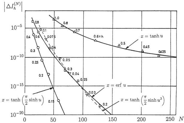
Figure 1. Comparison of the efficiency of several variable transformations for the integral \int_{-1}^1 dx / \{(x - 2)(1 - x)^{1/4}(1 + x)^{3/4}\} ; taken from Mori [5, Fig. 4] with permission from the European Mathematical Society; u and N in the figure correspond, respectively, to t and 2N + 1 in the present notation.
